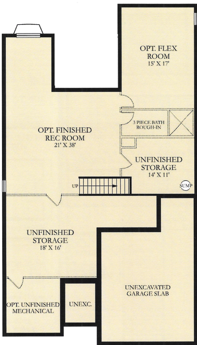
BASEMENT
